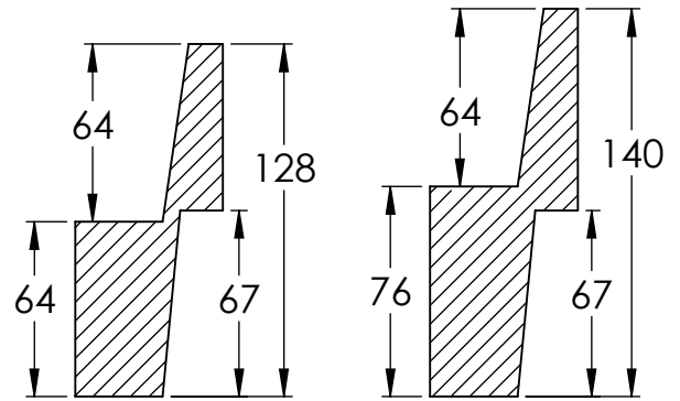
63.5mm (2.5") LIFT KR010-2.5
