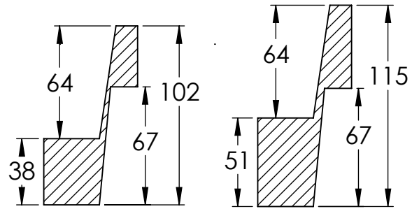
38mm (1.5") LIFT KR010-1.5
